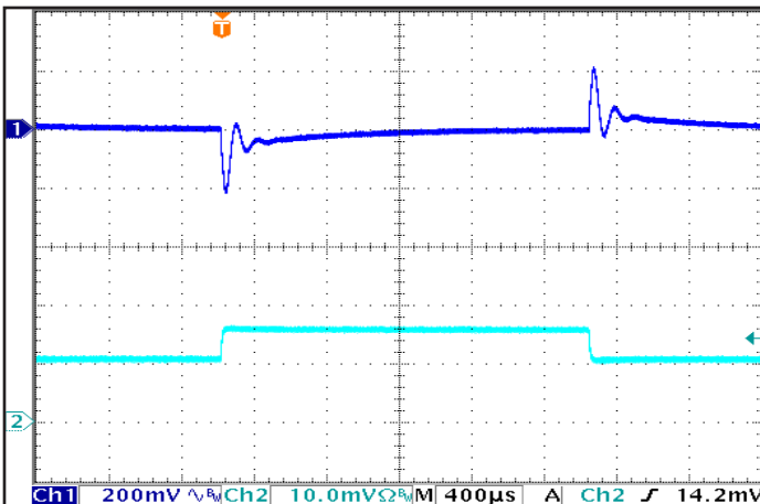
Figure 5: Output voltage response to step-change in load current (50%-75%-50% of I out (max); di/dt = 0.1 A/μs). Load cap: 1 μF ceramic and 15 μF tantalum capacitors. Ch 1: V out , Ch 2: I out (2A/div)
