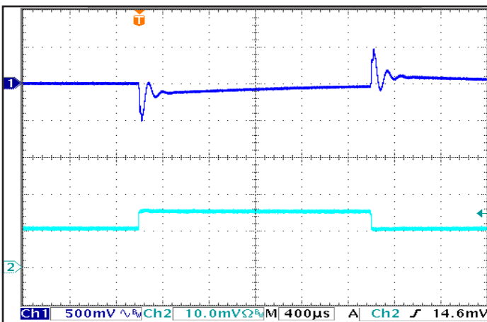
Figure 5: Output voltage response to step-change in load current (50%-75%-50% of I out (max); dI/dt = 0.1 A/μs). Load cap: 1 μF ceramic capacitor. Ch 1: V out , Ch 2: I out (1A/div).
