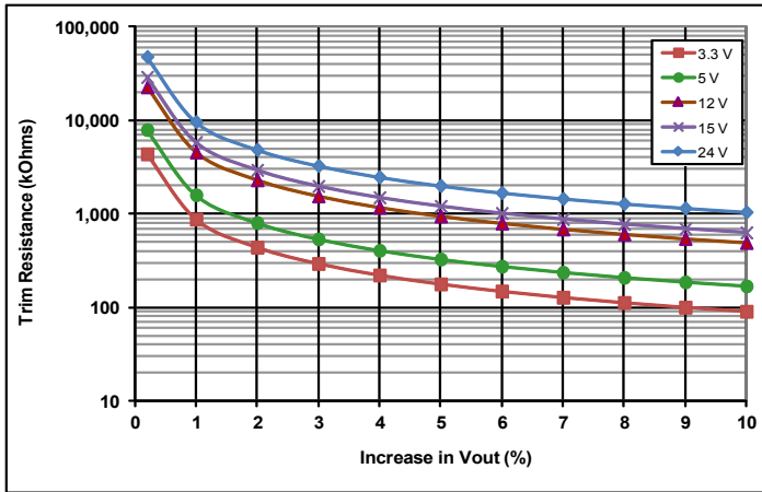
Common Figure 3: Trim graph for trim-up 3.3 to 24V outputs.
